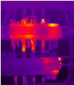
Electrical cabinet
